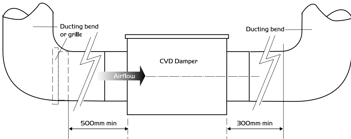
Figure 6. Installation practices to obtain the best result from the CVD damper.
