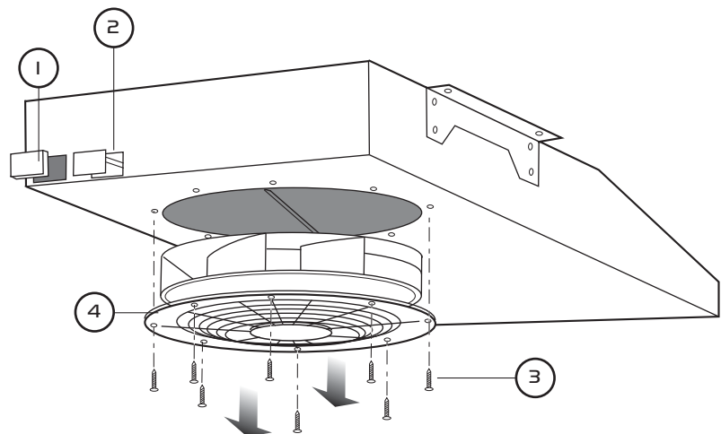
Figure 5. Impeller removal and dismantling.
