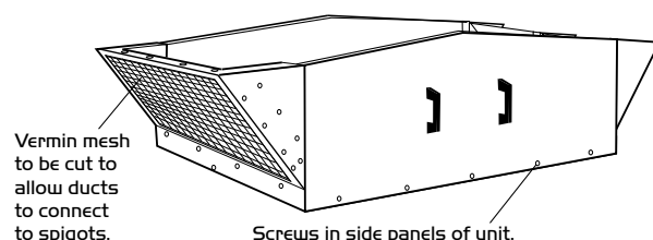
Figure 4. Having decided if one or both sides are to be removed from the unit, remove the screws in the side(s) of the unit with a flat screwdriver. The side(s) will then simply slide out.
