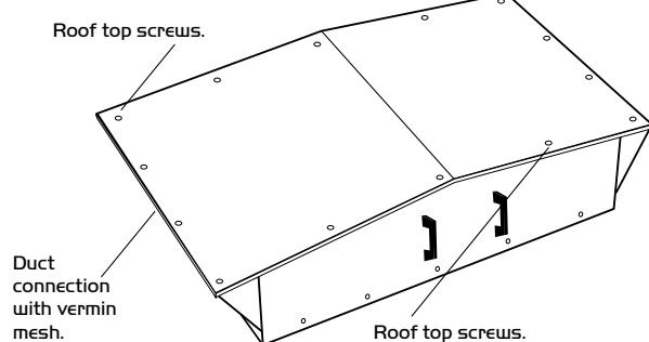
Figure 2. Remove the I4 Screws from the unit roof top which is riveted into one piece.
