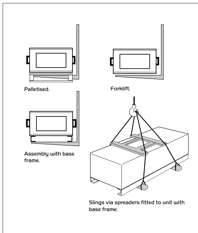
Figure 1. Methods of lifting.
