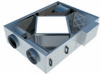
Model shown: S1-XB-RL (right hand with LPHW).
