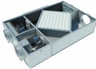
Model shown: XB2-5 and S6-XB-RN (right hand with no heater).
