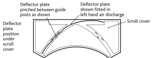
Deflector plate shown fitted for left hand air discharge (viewed from inside).
