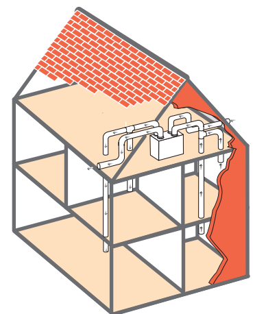
Typical installation with unit mounted in loft.
